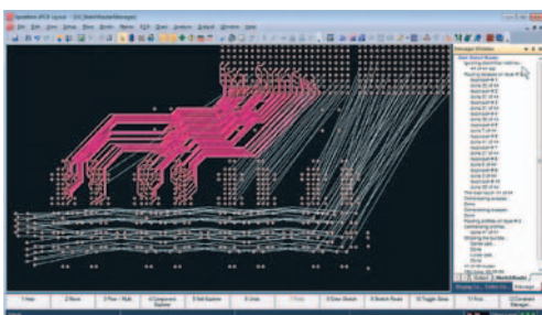
Sketch router
